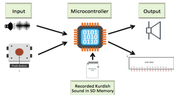
1.1 Block Diagram
